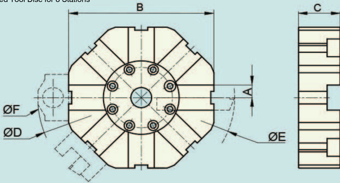
Slotted Tool Disc for 8 Stations
